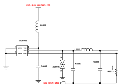
Sub MIC
