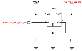
SENSOR LDO
